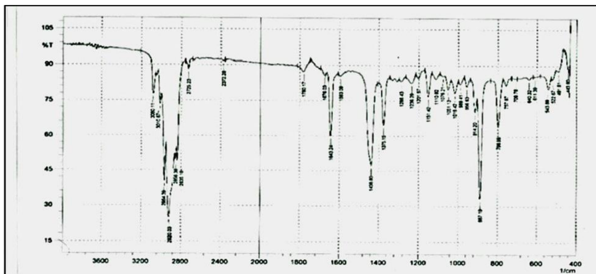
Figure 4: FTIR examination of C. aurantium essential oil compounds before silver nanoparticles formation
