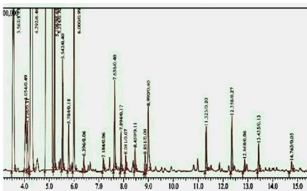
Figure 1: Typical GCMS chromatogram of C. aurantium essential oil.
