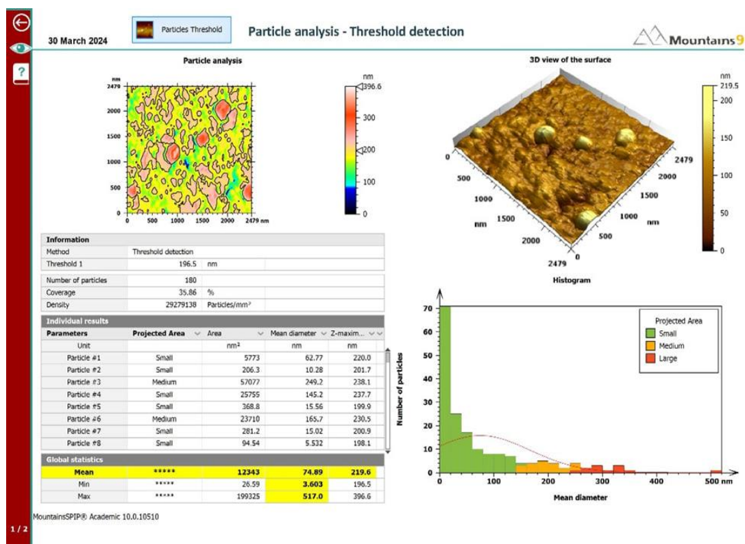
Figure 6: Average particle size of silver nanoparticles
