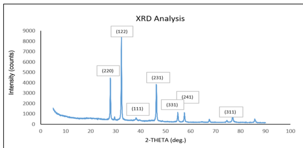
Figure 3: XRD analysis of fish mucus-mediated synthesised AgNPs
