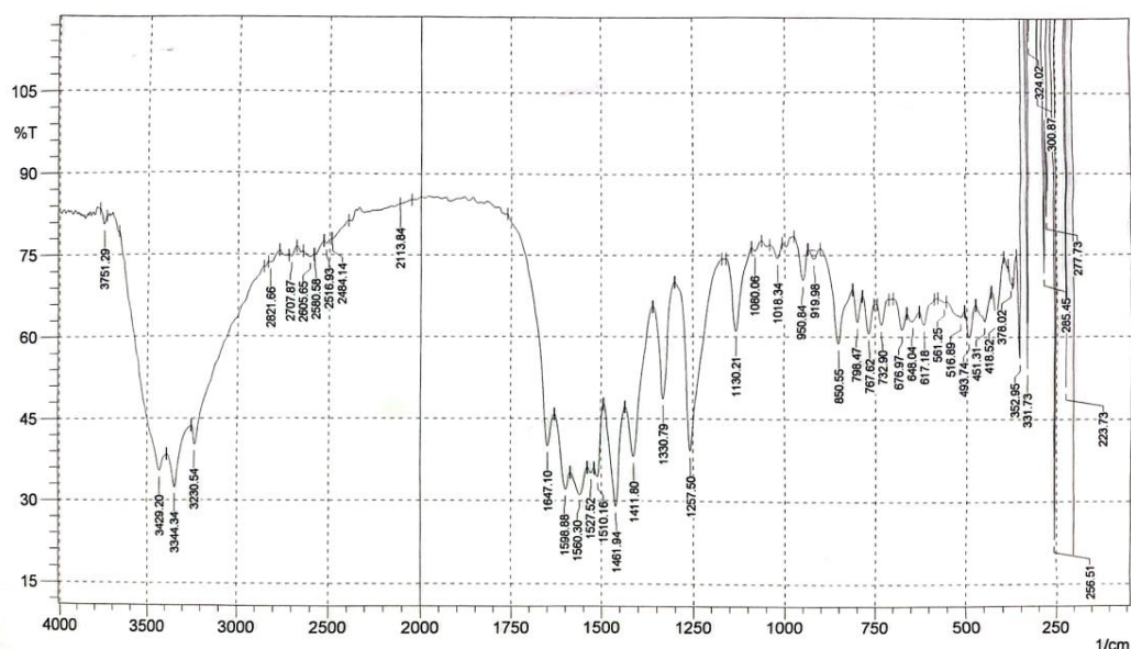
Figure 2: FTIR spectrum of BAE ligand
