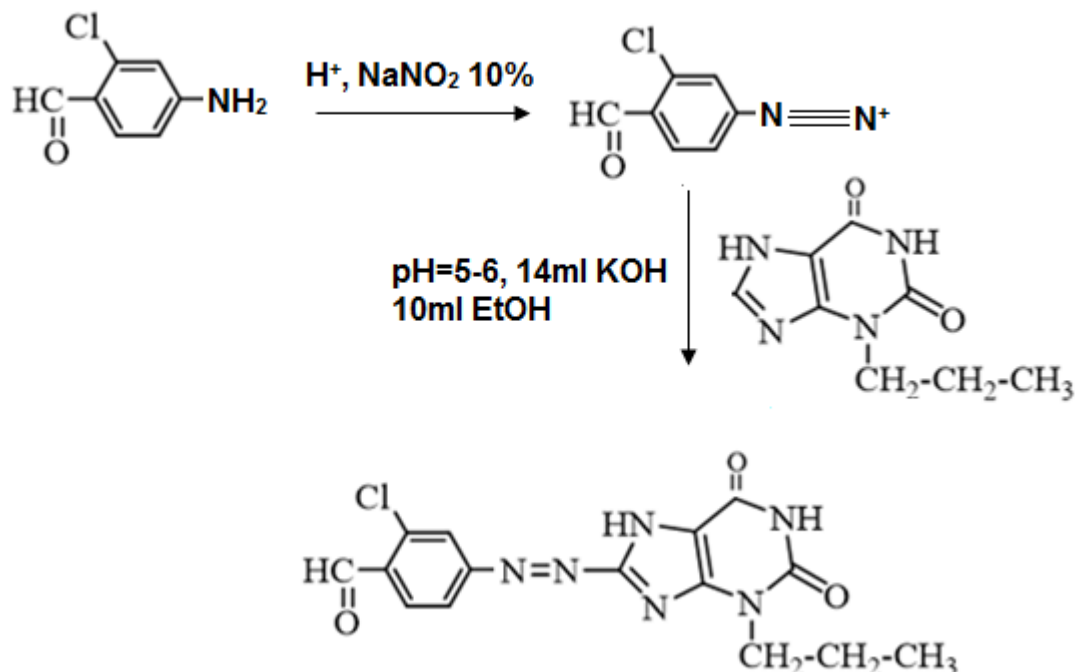
Scheme 1: A synthesis path of the ligand BAE
