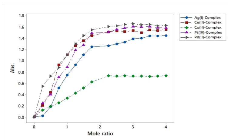
Figure 1: A Graph of mole ratio for BAE-Complexes
