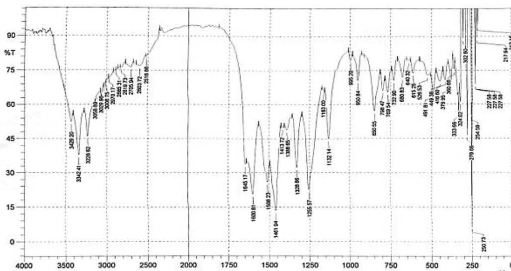
Figure3: FTIR spectrum of [Pt (BAE) 2 Cl 2 ]Cl 2 .H 2 O Complex.
