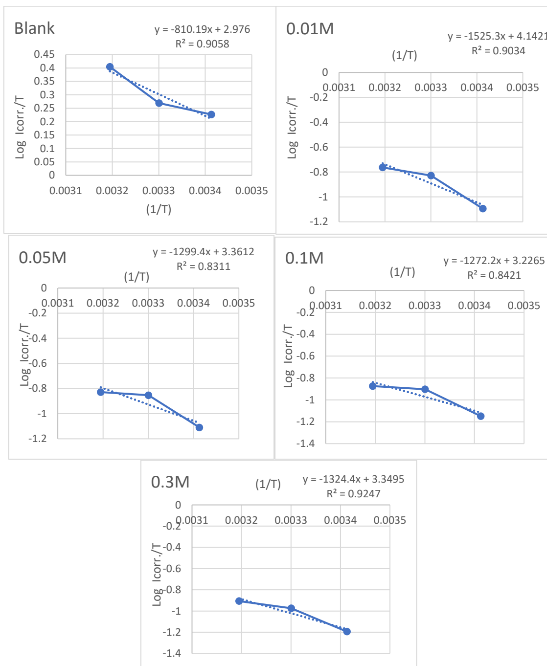
Figure 8: Arrhenius plots of \log I_{corr}/T against 1/T in the presence and absence of derivatives at concentrations of 0.01M, 0.05M, 0.1M, and 0.3M, measured at a range of temperatures For Compound (B).
