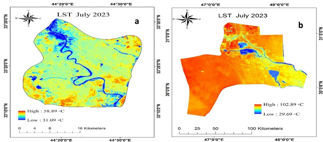
Figure 2 : LST in July 2023 (a) Baghdad, (b) Basrah
