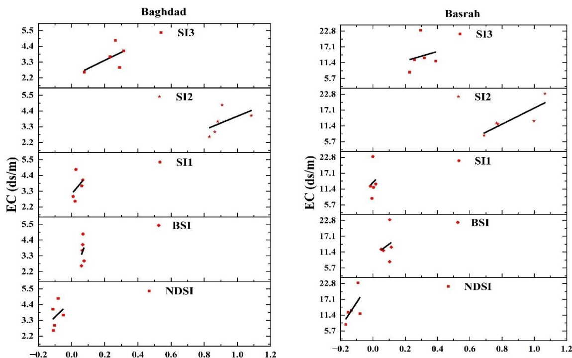
Figure 5: The relationship between Measured EC from ground truth and the salinity indices.
