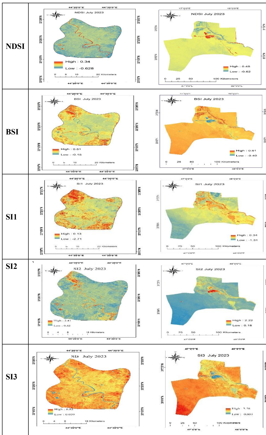
Figure :6 Salinity indices Maps of Baghdad and Basrah in July 2023, 1st row (NDSI), 2nd row (BSI), 3rd Row (SI1), 4th Row (SI2), and 5th Row (SI3).
