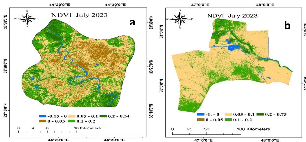
Figure 4: NDVI in July (a) Baghdad, (b) Basrah, 2023
