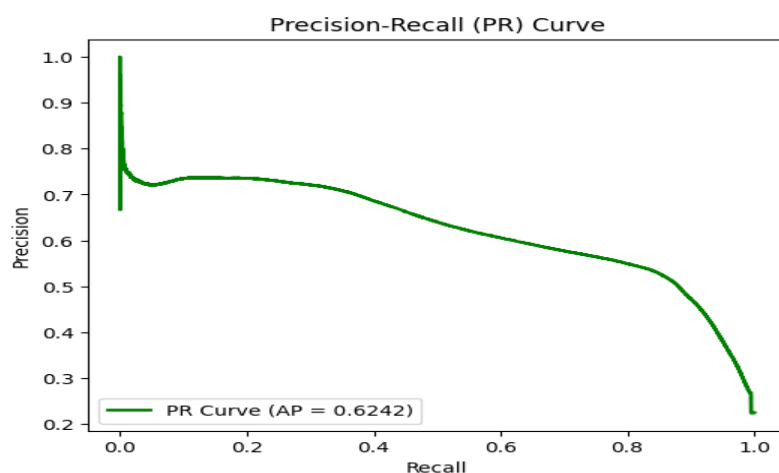
Figure 8: Precision-Recall Curve for Minutiae-SIFT.
