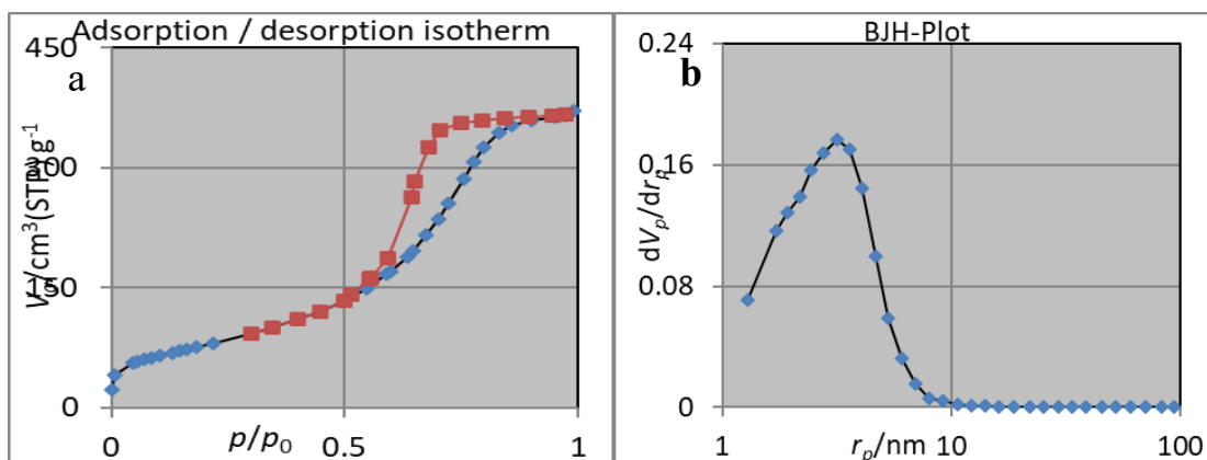
Figure 3: (a) \text{N}_2 adsorption/desorption isotherms and (b) \gamma -MNP pore-size distributions of \gamma -MNP
