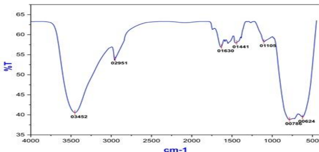
Figure 1: FTIR spectrum of \gamma -MNP after calcination
