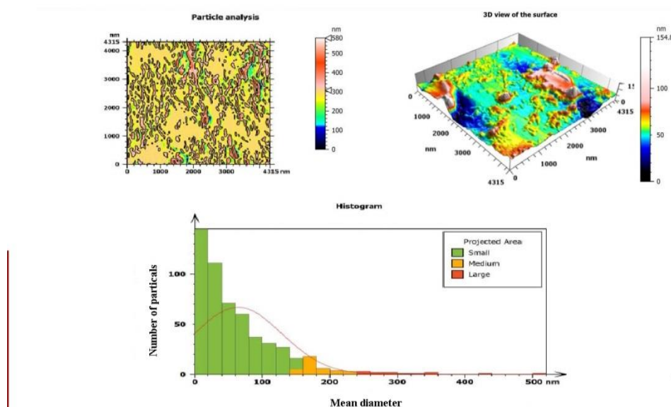
Figure 5: Histogram and distribution of granules and two- and three-dimensional view image for \gamma -MNP
